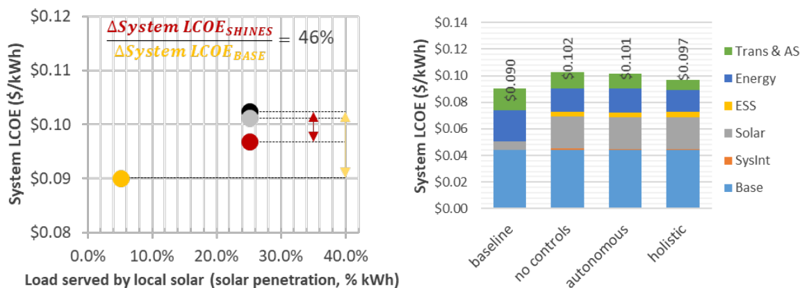
Figure 2-23 Scenario 14, Left: System LCOE results for each control strategy, Right: System LCOE breakdown
