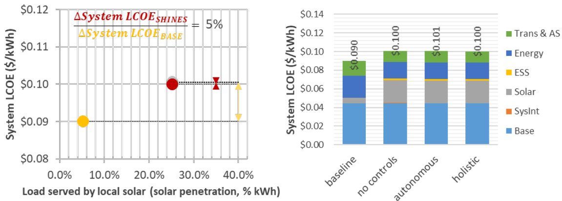
Figure 2-9 Scenario 7, Left: System LCOE results for each control strategy, Right: System LCOE breakdown
