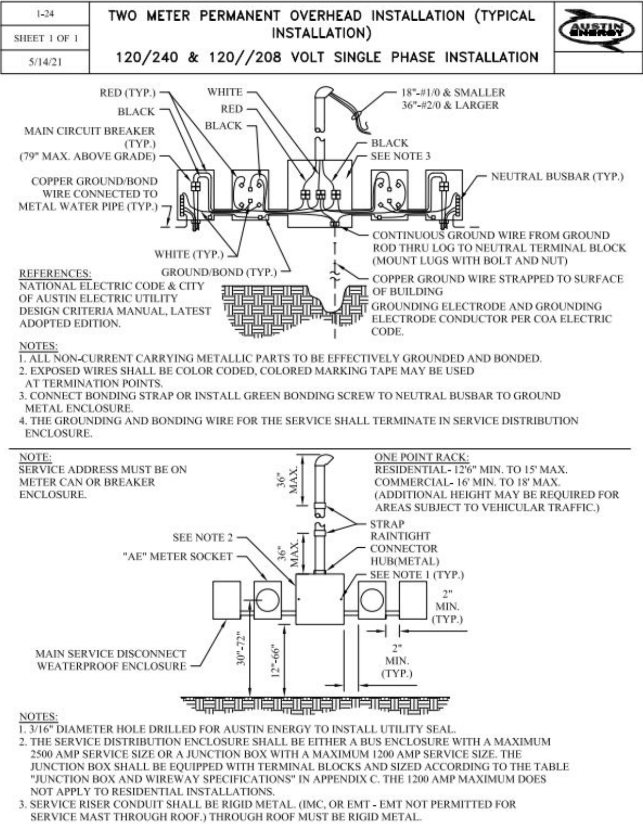
Figure 1-24. Two-Meter Permanent Overhead Installation (Typical Installation)
