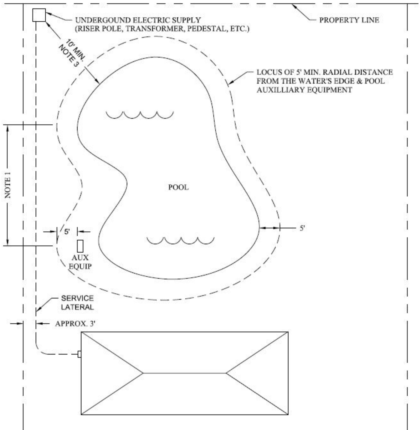
Figure 1.10.7B - Clearance from Water Holding Facilities to Underground Electric Facilities
