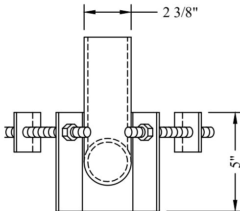
POLE MOUNT P/M FLOODLIGHT MOUNTING BRAKET 1928-60-05
