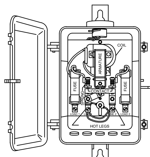
DOUBLE POLE 60A RELAY 1928-55-25
