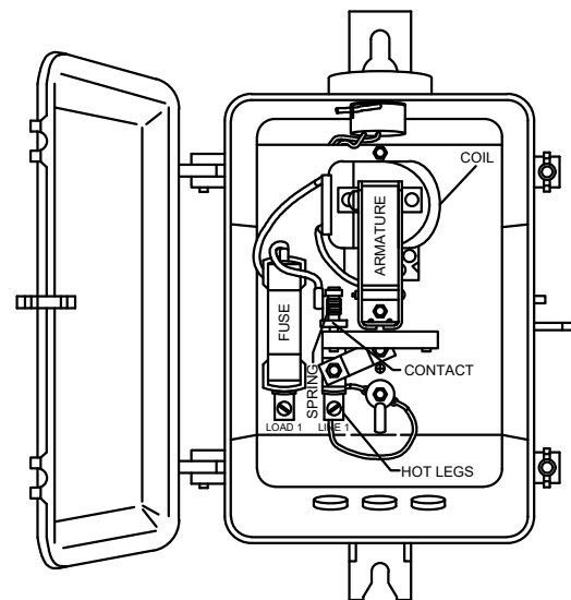
SINGLE POLE 60A RELAY 1928-55-20
