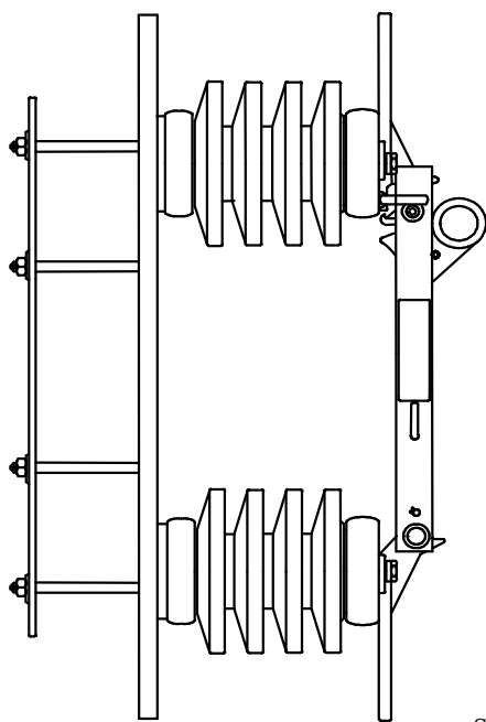
1370-05-01 FRONT VIEW
