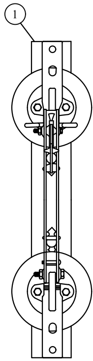
1370-05-01 FRONT VIEW
