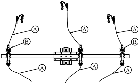
8-FOOT/10-FOOT DEAD-END ARM 1368-12-20 1368-12-21 1368-12-22 1368-12-24 1368-12-25
