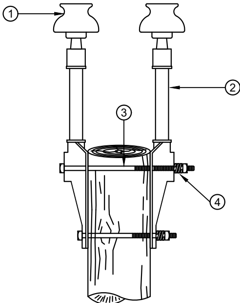
SIDE VIEW
