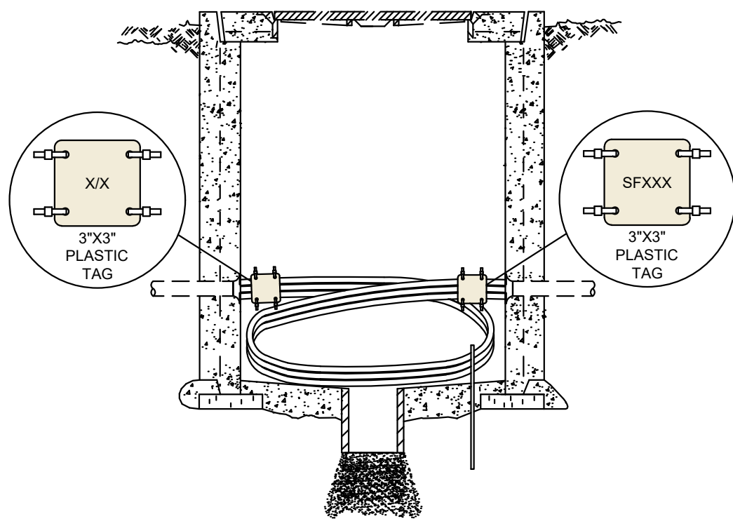
36" PULLBOX THREE PHASE URD (PRIMARY)
