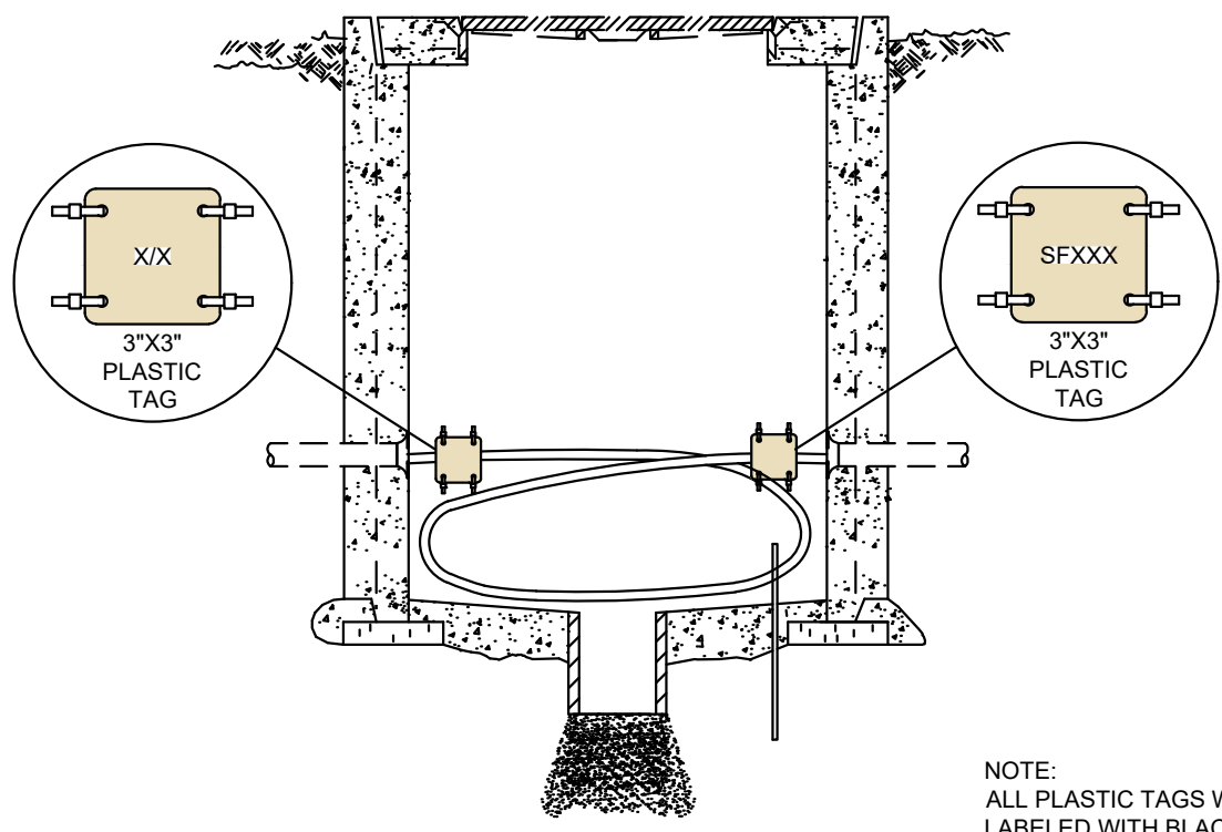
36" PULLBOX SINGLE PHASE URD (PRIMARY)
