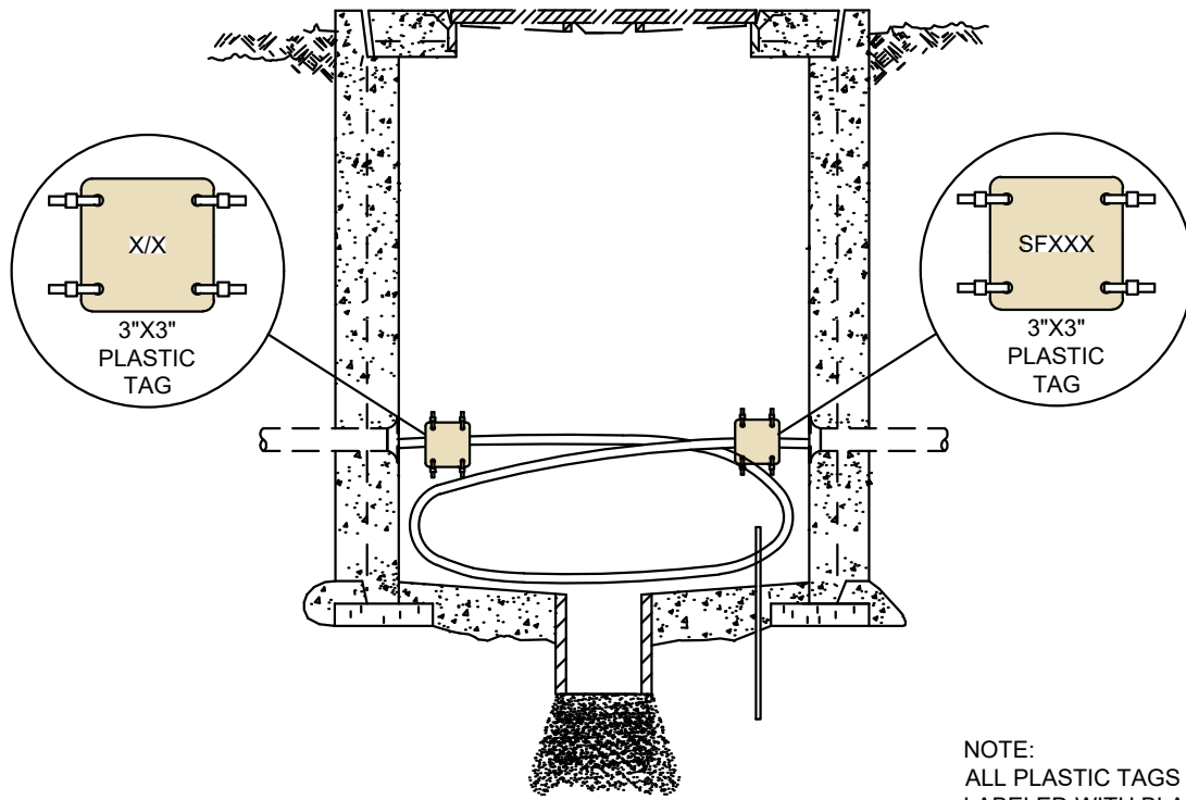
36" PULLBOX SINGLE PHASE URD (PRIMARY)
