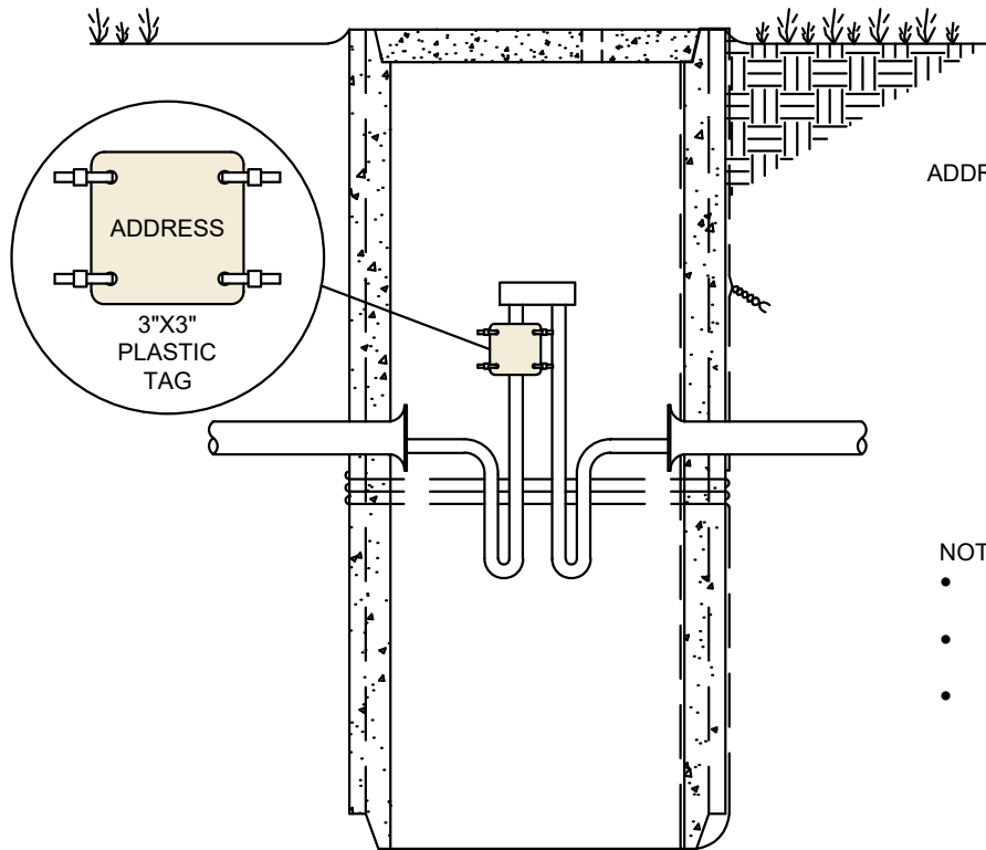
18" SERVICE BOX SINGLE SERVICE
