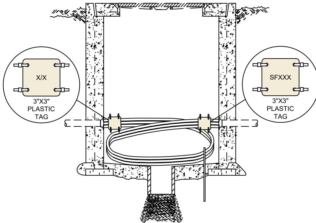
36" PULLBOX THREE PHASE URD (PRIMARY)
