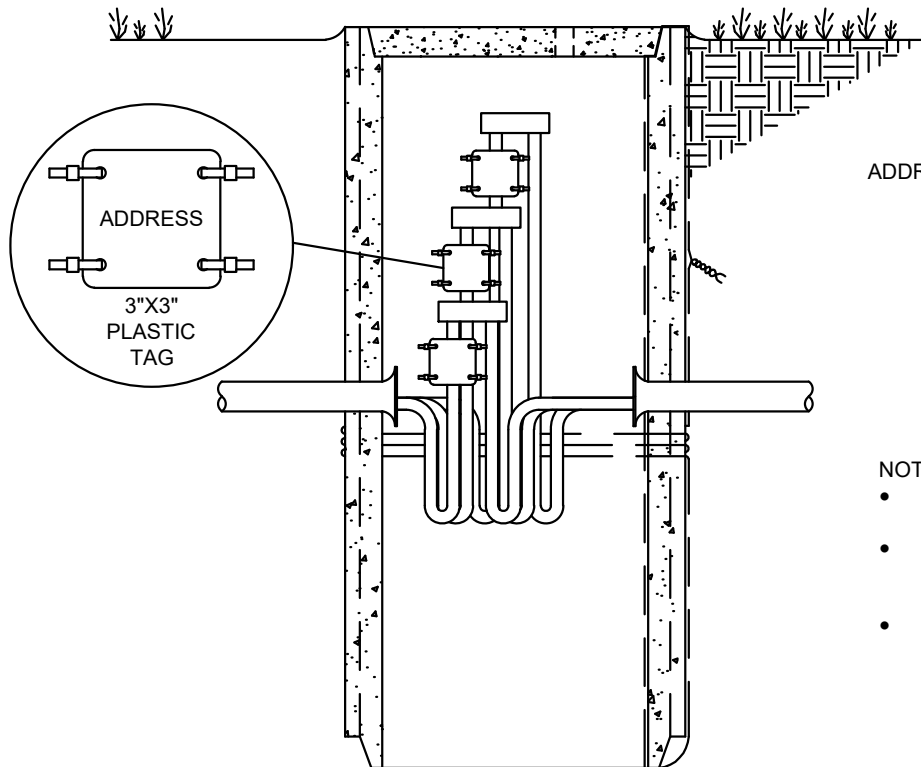
18" SERVICE BOX MULTIPLE SERVICE
